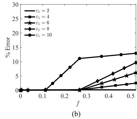
FIGURE 3. Limitation of Maxwell Garnett (2) [19]. (a) Comparison of the simulated and calculated \epsilon_{eff} for different values of \epsilon_1 when \epsilon_2 = 1 . (b) Permittivity perceptual error (%) as a function of f .
